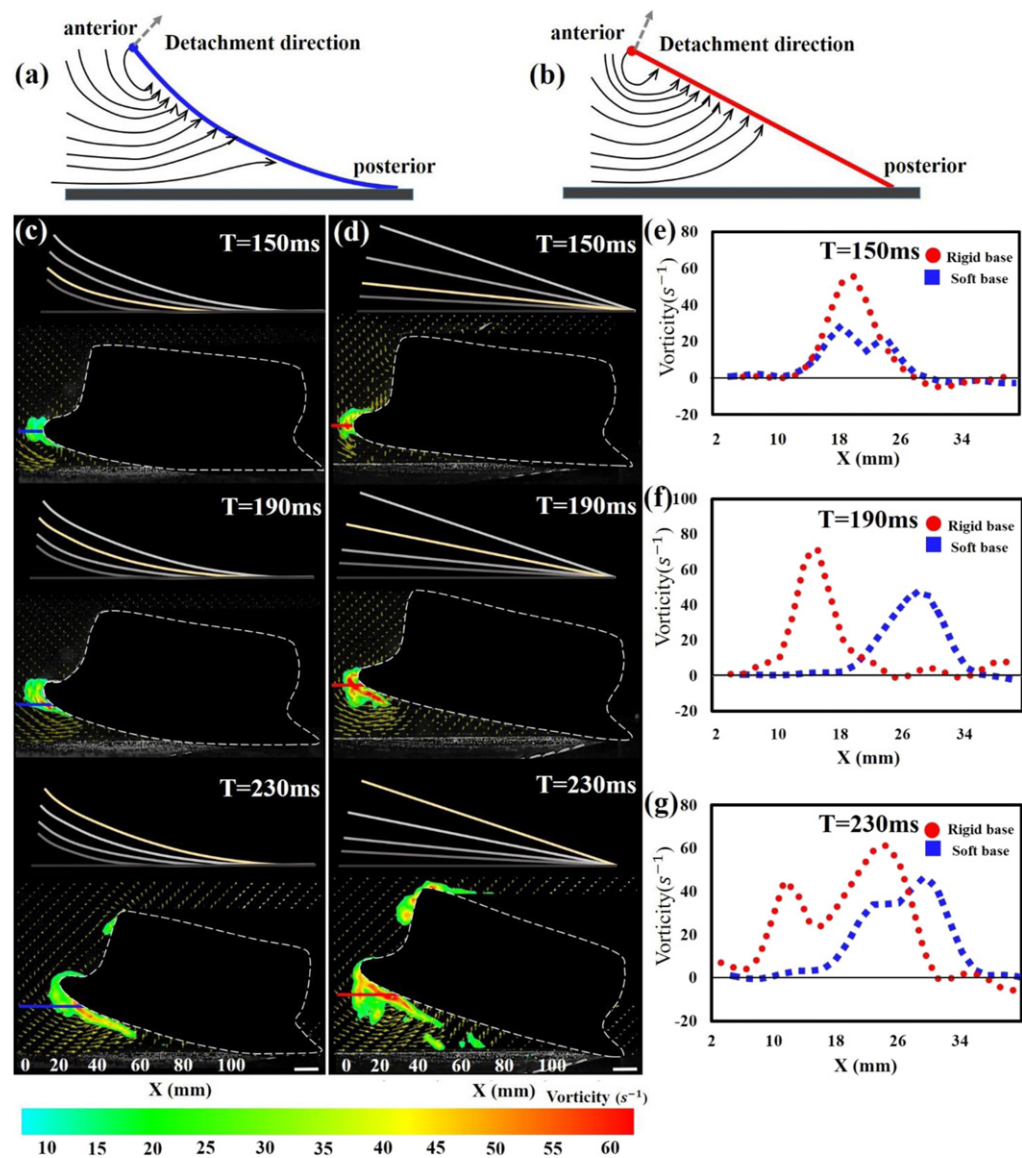
Figure 8. DPIV vorticity analysis of the soft-base and the rigid-base discs during the raising process of stage 2. Schematic diagrams (the profiles were depicted from the streamline of the flow calculated by particle tracer method) of the leading-edge vortex (LEV) generated by the discs with the soft-base (a) and the rigid-base (b) during the raising process. The gray arrow indicates the direction of the velocity of the disc's leading edge. (c) DPIV images of the soft-base disc and (d) the rigid-base disc at different instants: 150 ms, 190 ms and 230 ms. The superimposed solid lines above the DPIV images indicate the profiles of the disc lip (from side view shown in the DPIV images) at different time intervals. The yellow lines correspond to the time of the DPIV image. Scale bar: 1 cm. Values for the vorticity of the leading-edge vortex near both rigid and soft discs' surfaces were taken along the red and blue line transects from the disc surface into the flow and are plotted against x -axis along the transect at different time instants (e) 150 ms (f) 190 ms (g) 230 ms.
